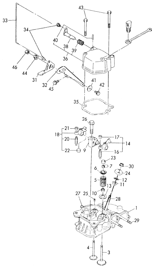
Fig.49 CYLINDER HEAD
