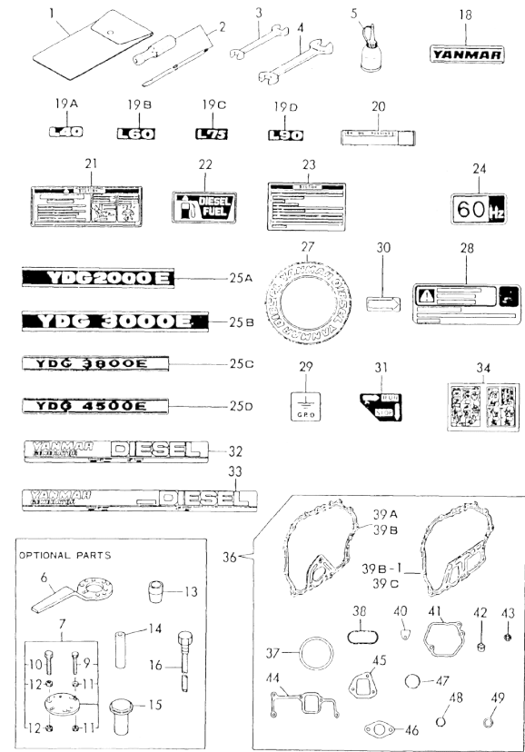
Fig.10 TOOLS/LABELS & GASKET SET
