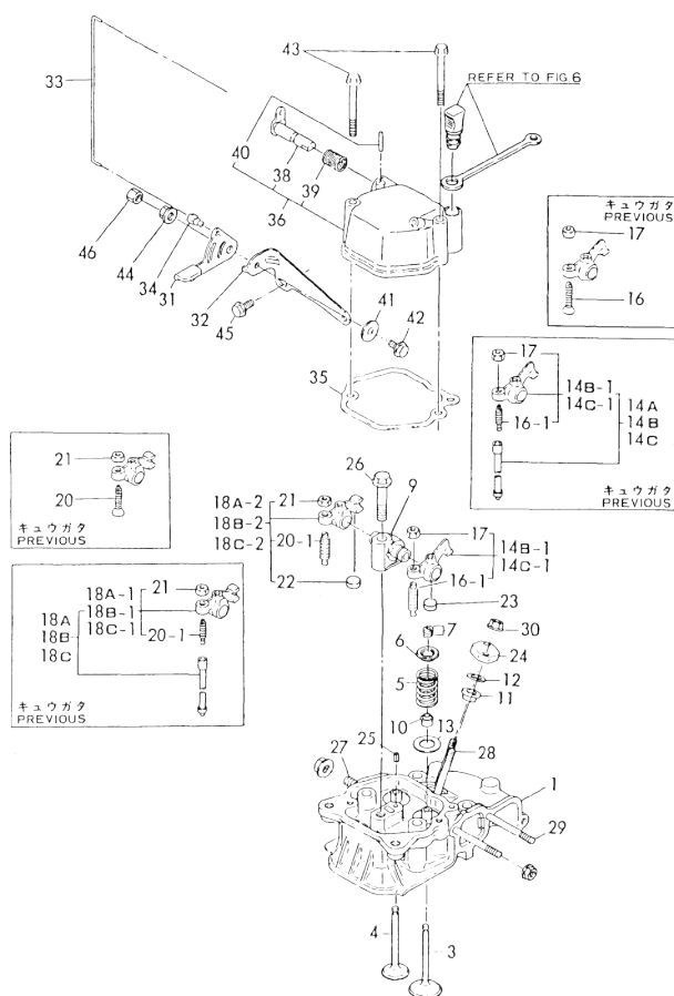
Fig. 2 CYLINDER HEAD
