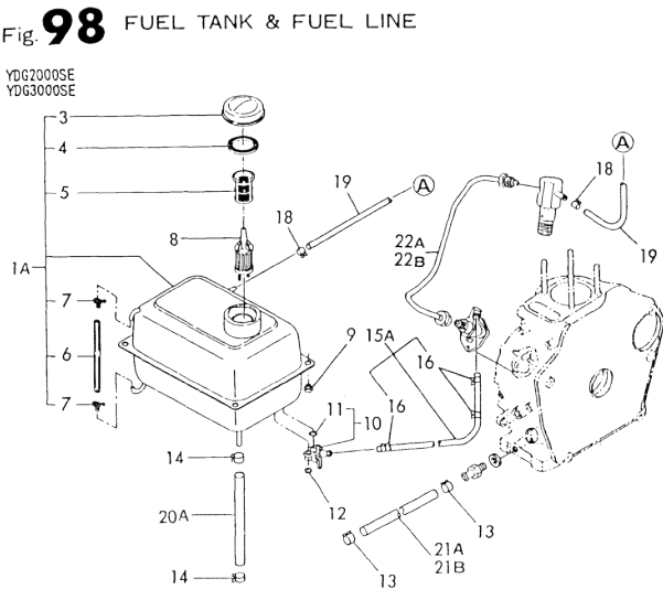
Fig.98. FUEL TANK & FUEL LINE
