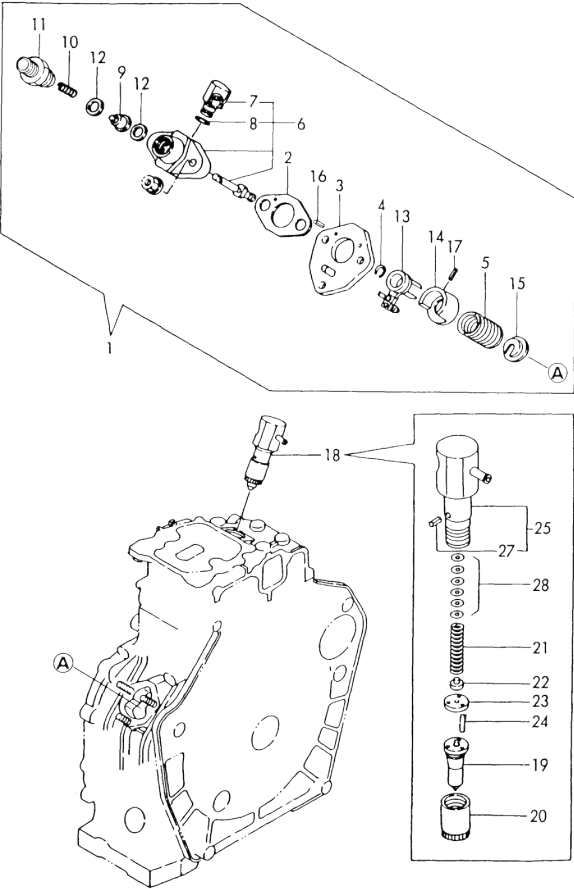
Fig.7 FUEL INJECTION PUMP & VALVE
