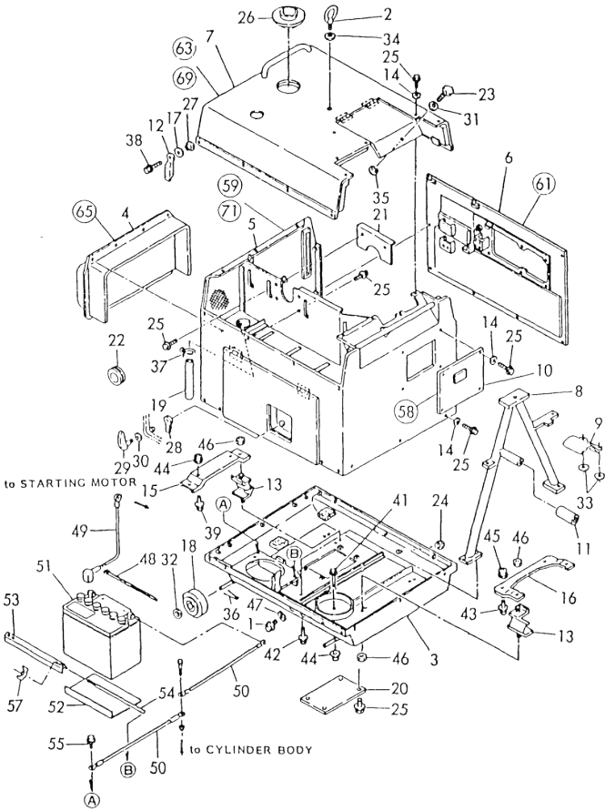
Fig. 117 SOUND-PROOF CASE
