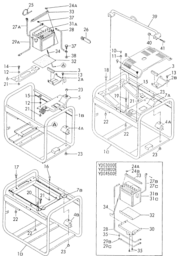
Fig. 11 FRAME & BATTERY
