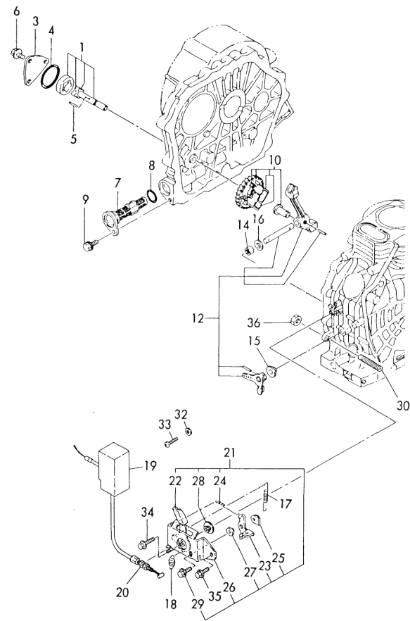
Fig.52 L. O PUMP & ENGINE CONTROL
