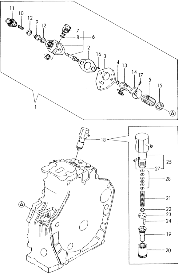
Fig. 38 FUEL INJECTION PUMP & VALVE
