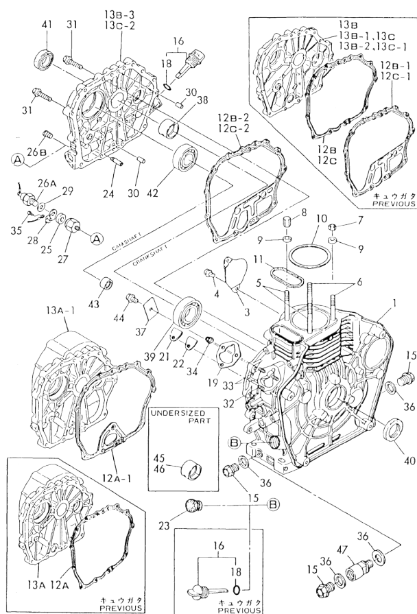
Fig. 78 CYLINDER BLOCK
