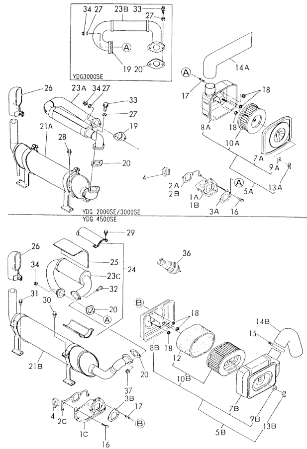
Fig. 109 AIR CLEANER & SILENCER
