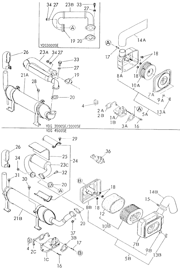
Fig. 93 AIR CLEANER & SILENCER
