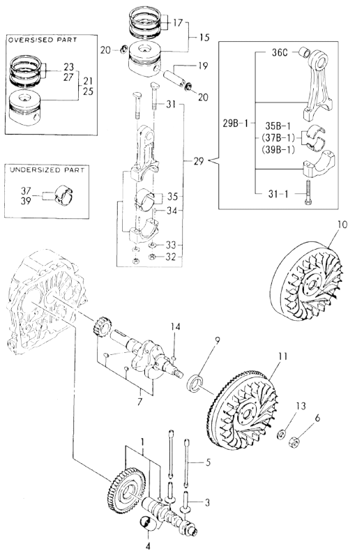
Fig.66 CRANKSHAFT / PISTON / ROD
