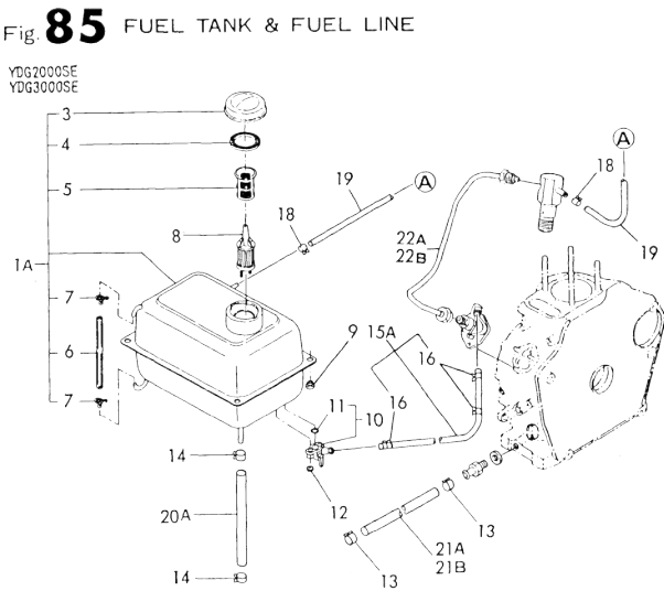
Fig.85. FUEL TANK & FUEL LINE
