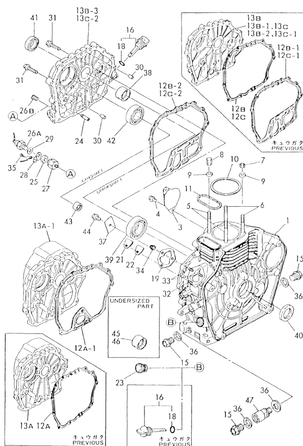
Fig. 78 CYLINDER BLOCK
