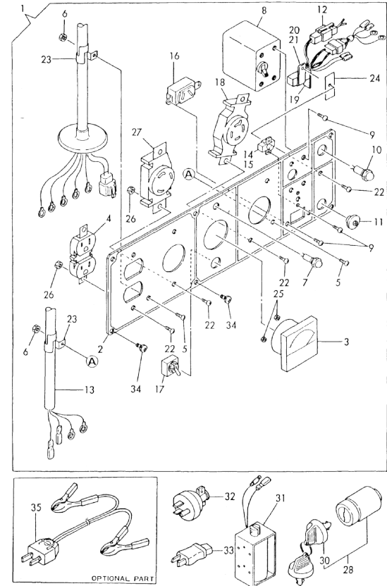
Fig. 121 PANEL
