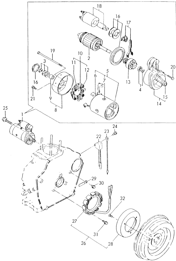
Fig.57 STARTING MOTOR & DYNAMO
