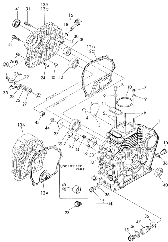
Fig.32 CYLINDER BLOCK
