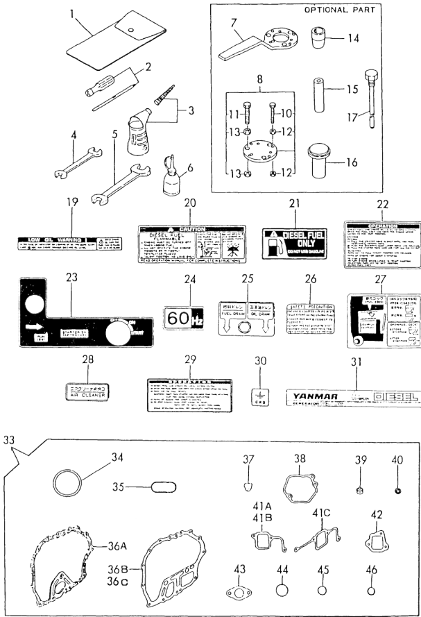
Fig.116 TOOLS/LABELS & GASKET SET
