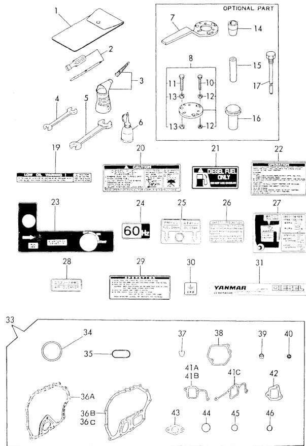
Fig.87 TOOLS/LABELS & GASCKET SET
