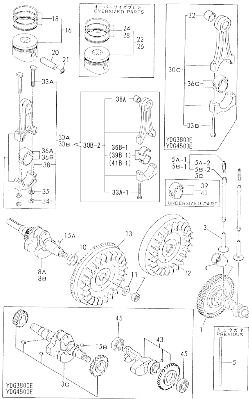
Fig.4 CRANKSHAFT/PISTON/ROD
