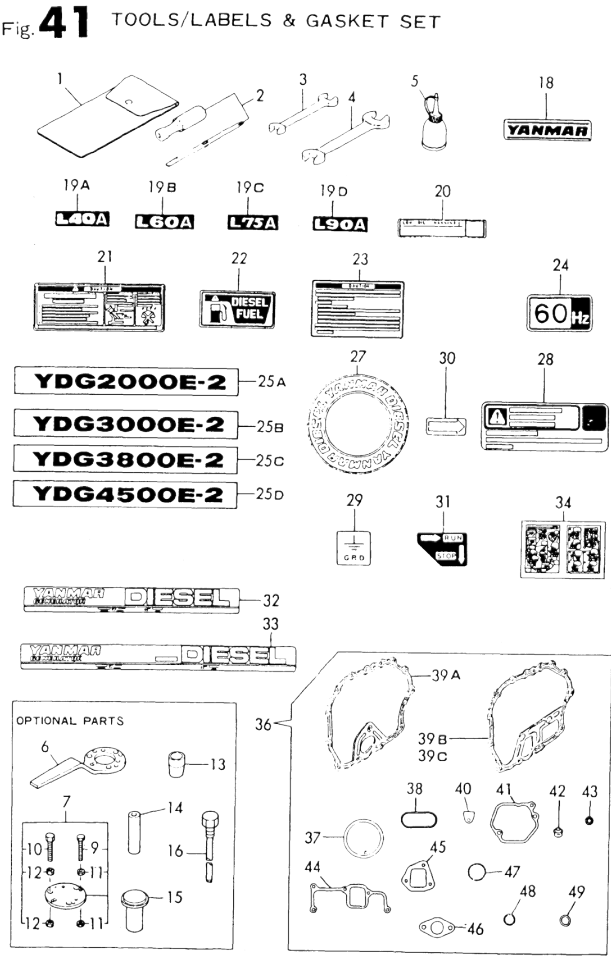
Fig.41. TOOLS / LABELS / GASKET SET
