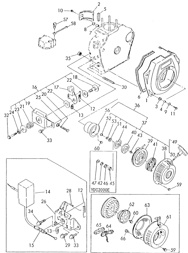
Fig. 37 COOLING & STARTING DEVICE
