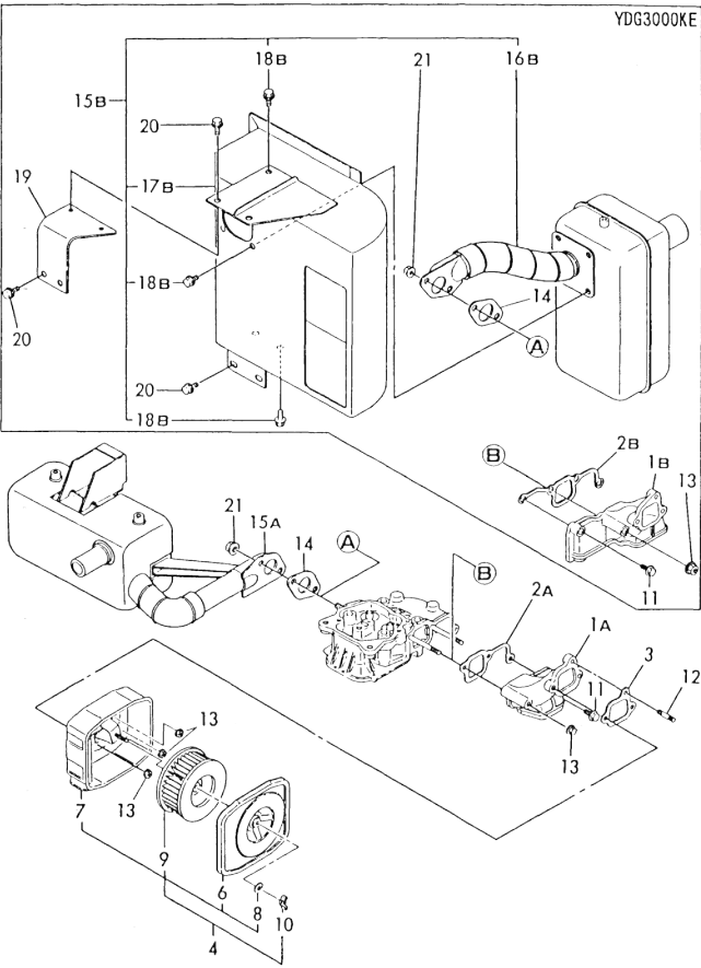
Fig. 65 AIR CLEANER & SILENCER
