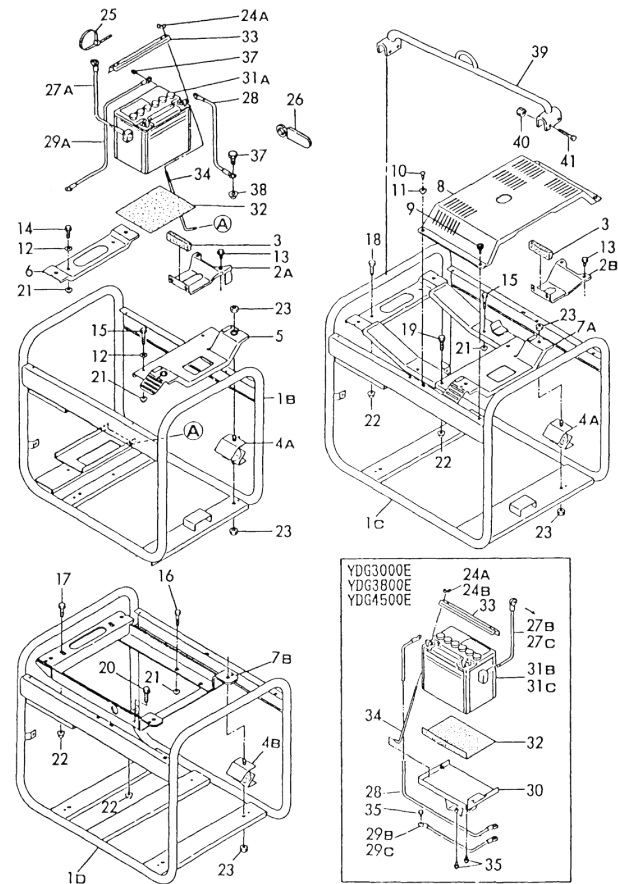
Fig.42 FRAME & BATTERY
