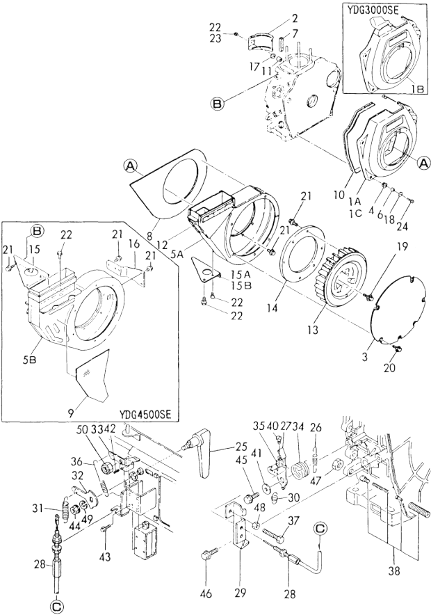
Fig.83 COOLING & ENGINE CONTROL
