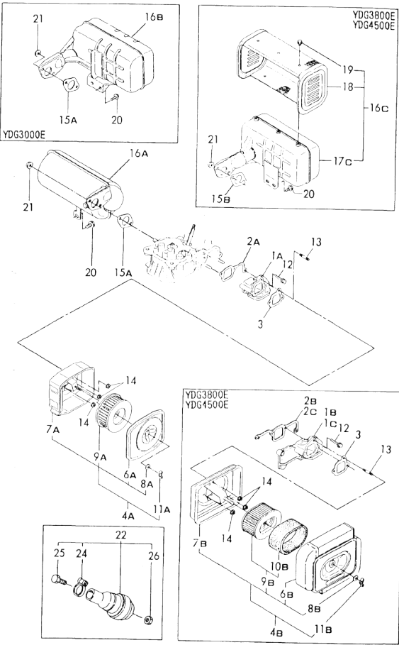
Fig.18 AIR CLEANER & SILENCER
