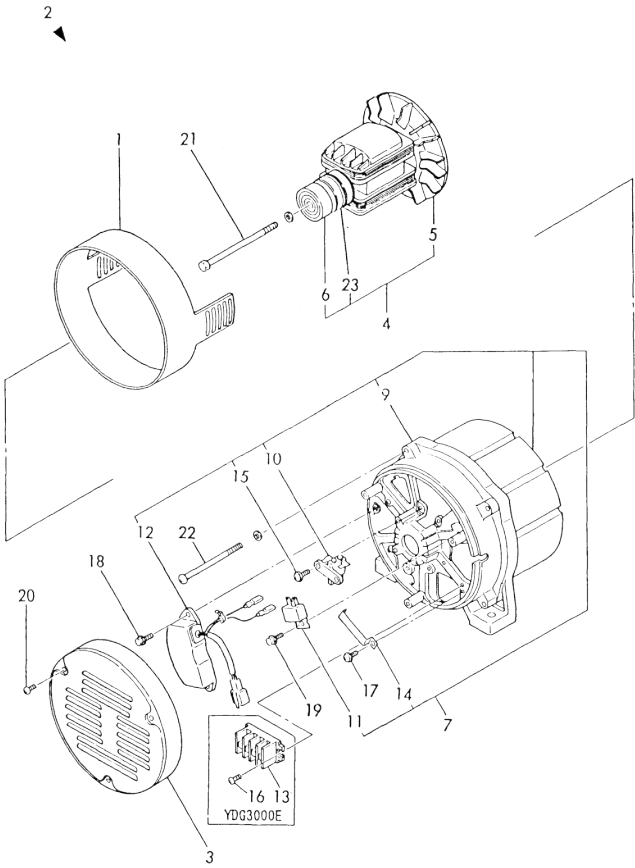
Fig.61 GENERATOR
