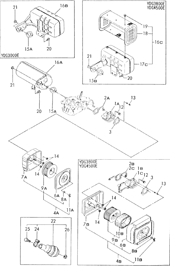
Fig. 34 AIR CLEANER & SILENCER
