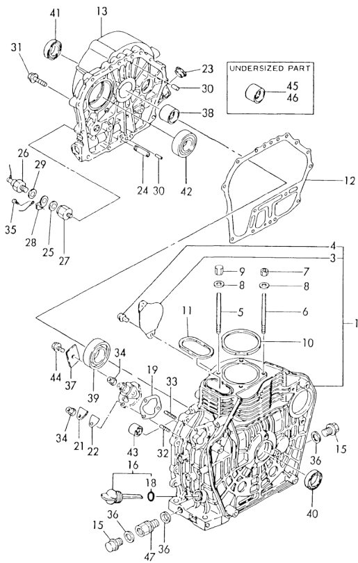
Fig.63 CYLINDER BLOCK
