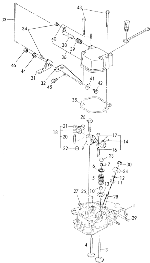
Fig. 17 CYLINDER HEAD
