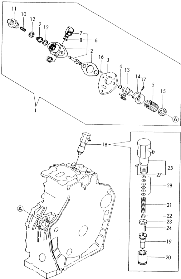
Fig. 22 FUEL INJECTION PUMP & VALVE
