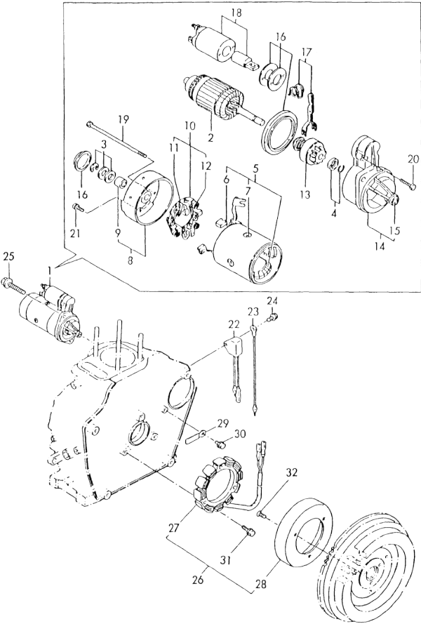
Fig.99 STARTING MOTOR & DYNAMO
