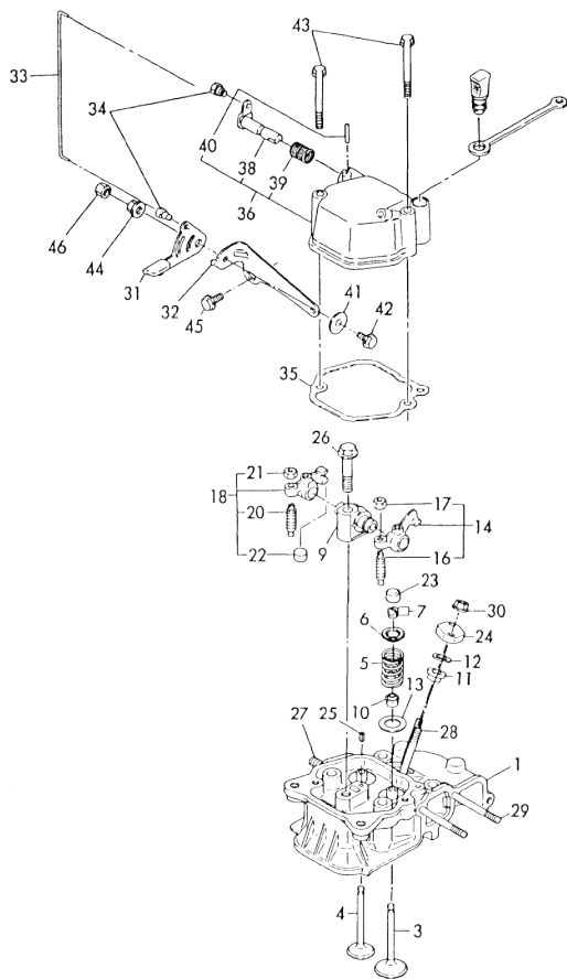
Fig. 92 CYLINDER HEAD
