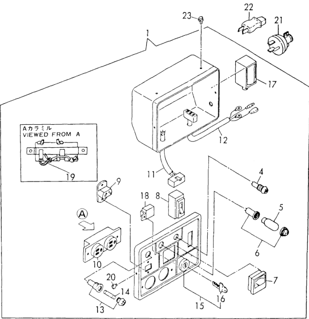
Fig.46 PANEL BOX
