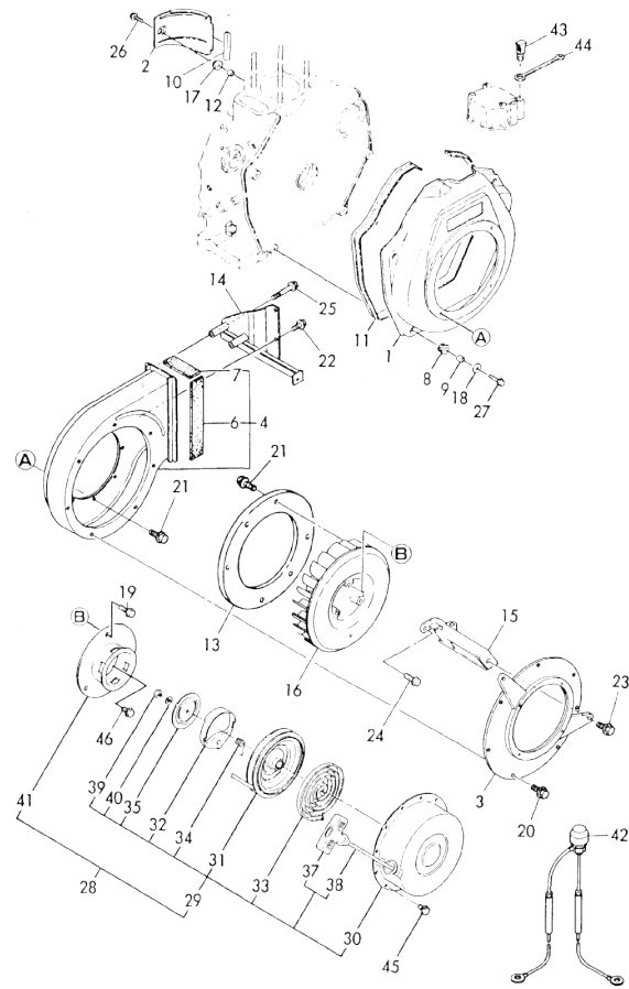
Fig.54 COOLING & STARTING DEVICE
