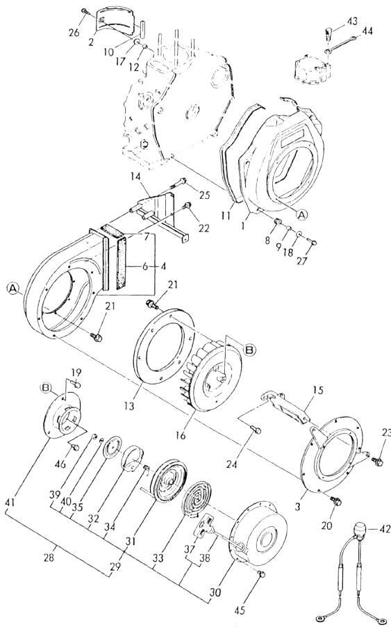
Fig. 69 COOLING & STARTING DEVICE
