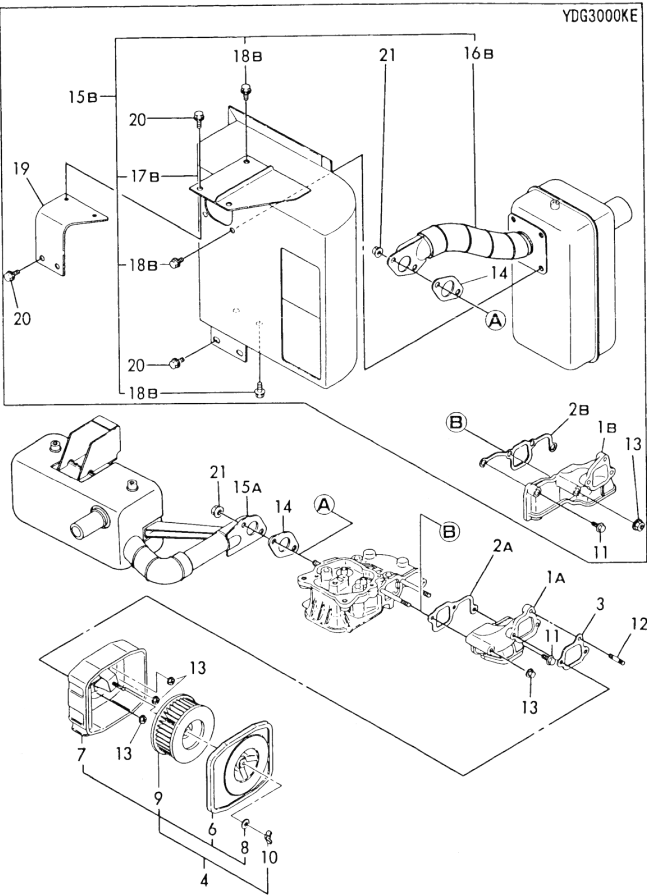
Fig.50 AIR CLEANER & SILENCER
