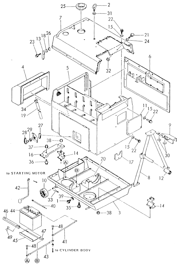
Fig. 102 SOUND-PROOF CASE
