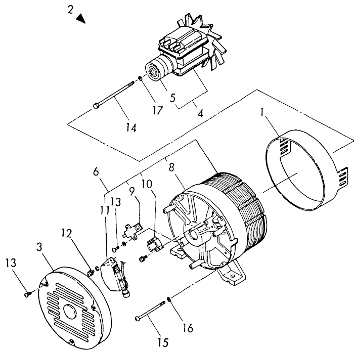
Fig.89 GENERATOR
