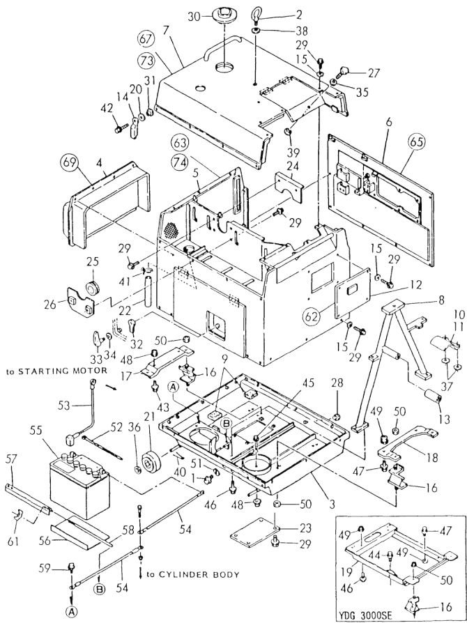
Fig. 88 SOUND-PROOF CASE
