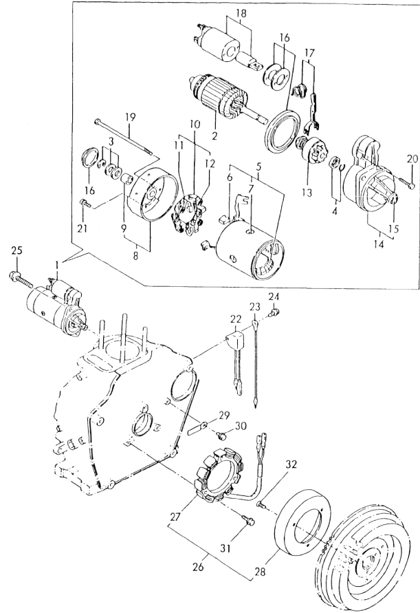
Fig.86 STARTING MOTOR & DYNAMO
