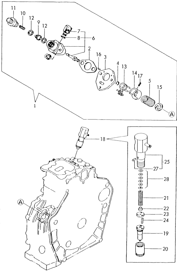
Fig.84 FUEL INJECTION PUMP & VALVE
