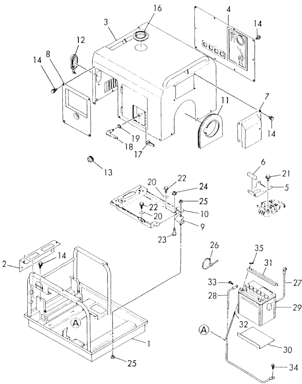
Fig.60 SOUND-PROOF CASE
