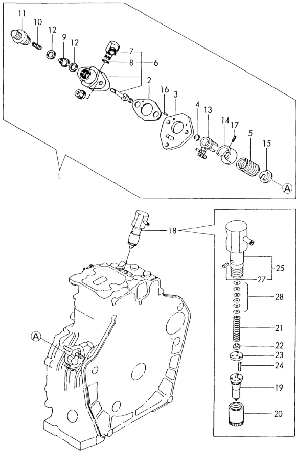
Fig. 97 FUEL INJECTION PUMP & VALVE
