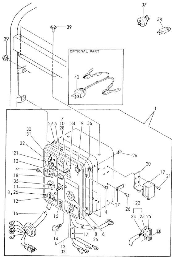
Fig.47 PANEL BOX
