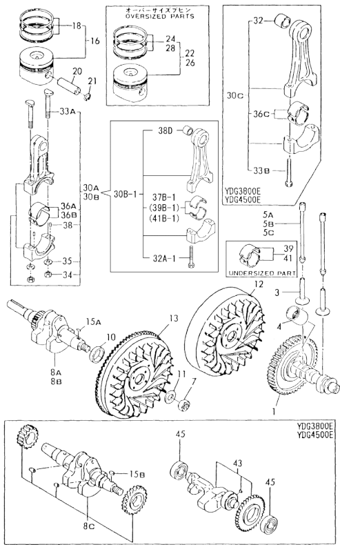
Fig. 110 CRANKSHAFT / PISTON/ROD
