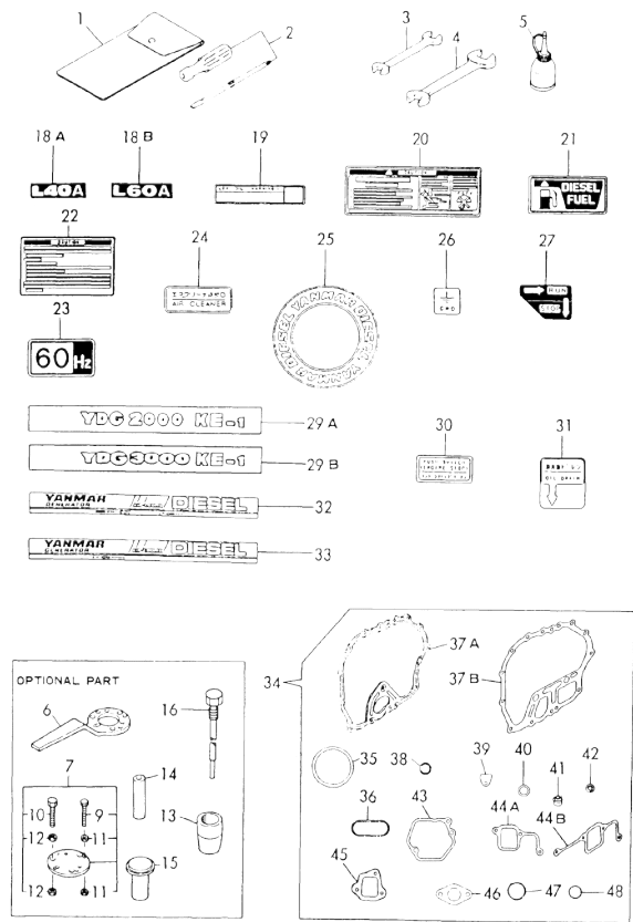
Fig.73 TOOLS/LABELS & GASKET SET
