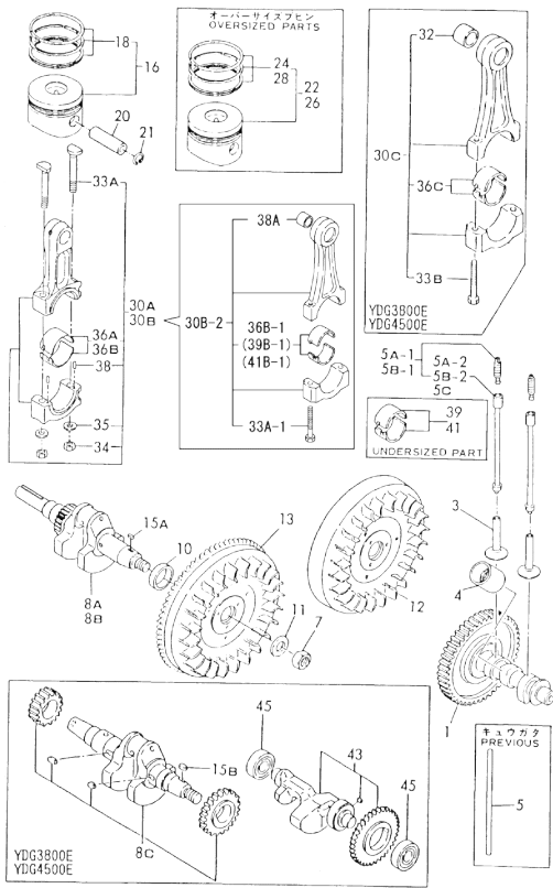
Fig.4 CRANKSHAFT/PISTON/ROD
