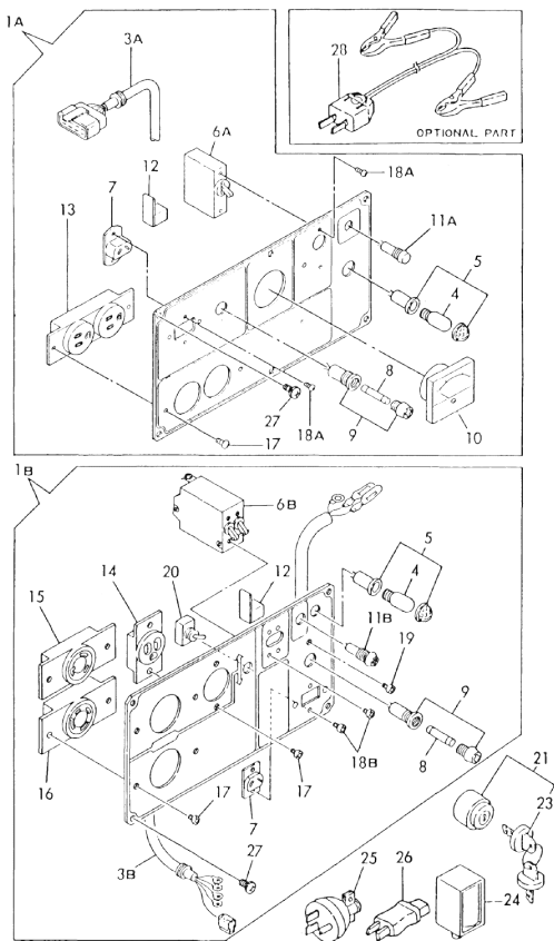
Fig.122 PANEL
