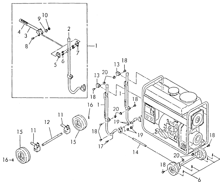
Fig. 43 WHEEL (OPTIONAL PARTS)
