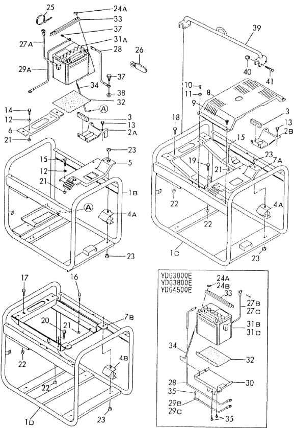
Fig.26 FRAME & BATTERY
