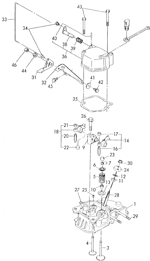
Fig. 108 CYLINDER HEAD
