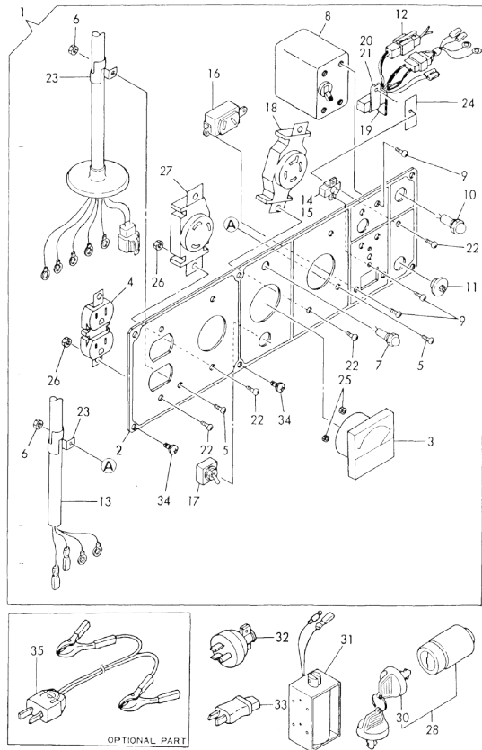
Fig. 106 PANEL
