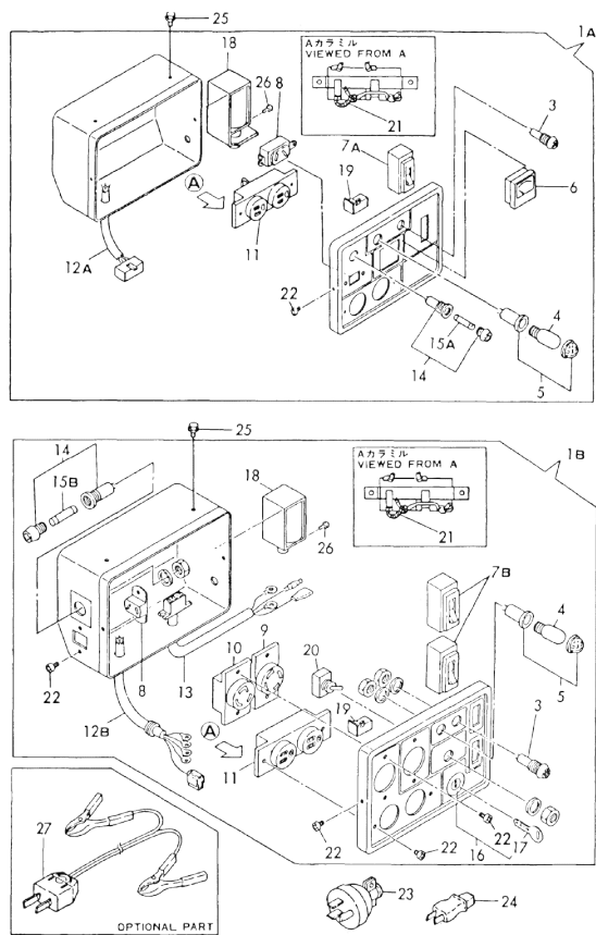
Fig. 62 PANEL BOX
