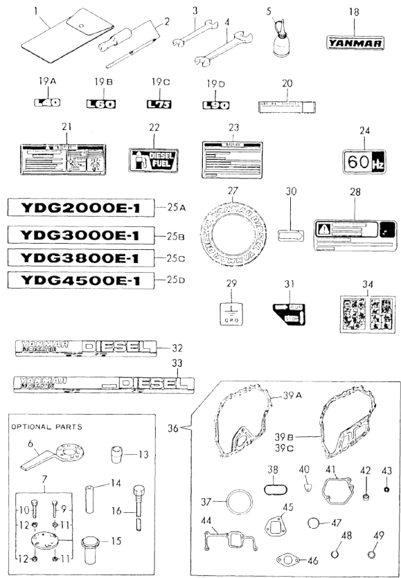
Fig.25 TOOLS/LABELS & GASKET SET
