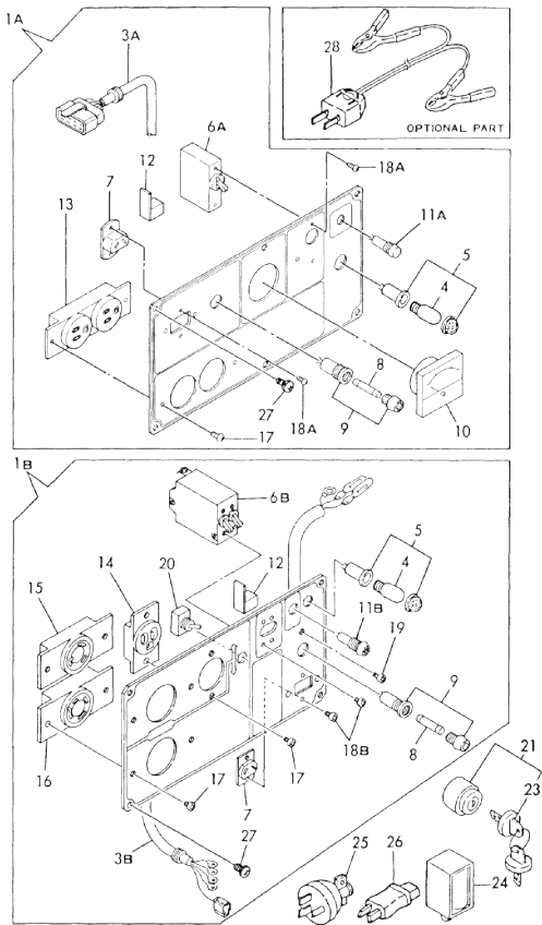
Fig. 105 PANEL
