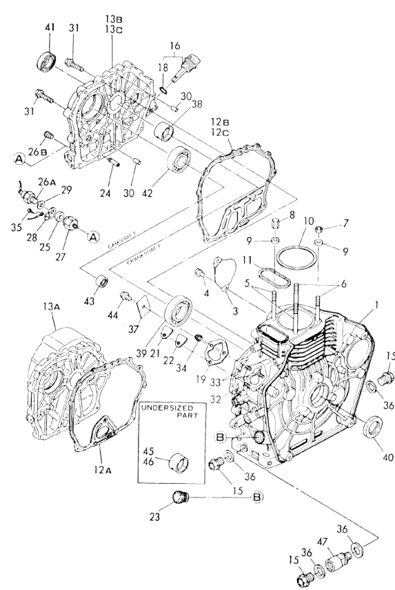
Fig. 16 CYLINDER BLOCK
