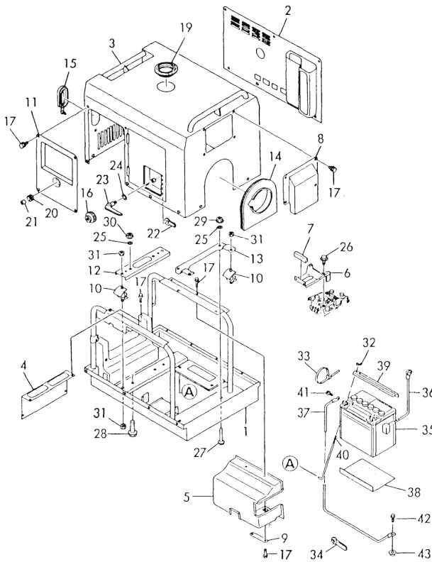
Fig.74 SOUND-PROOF CASE
