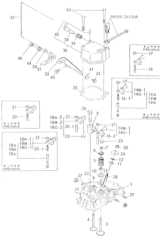
Fig.2 CYLINDER HEAD
