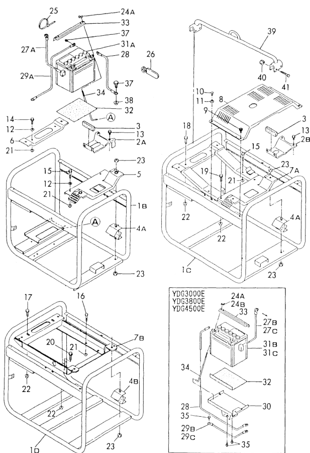
Fig. 11 FRAME & BATTERY
