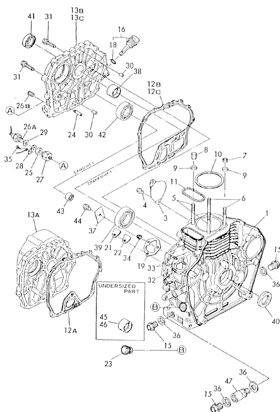
Fig. 91 CYLINDER BLOCK
