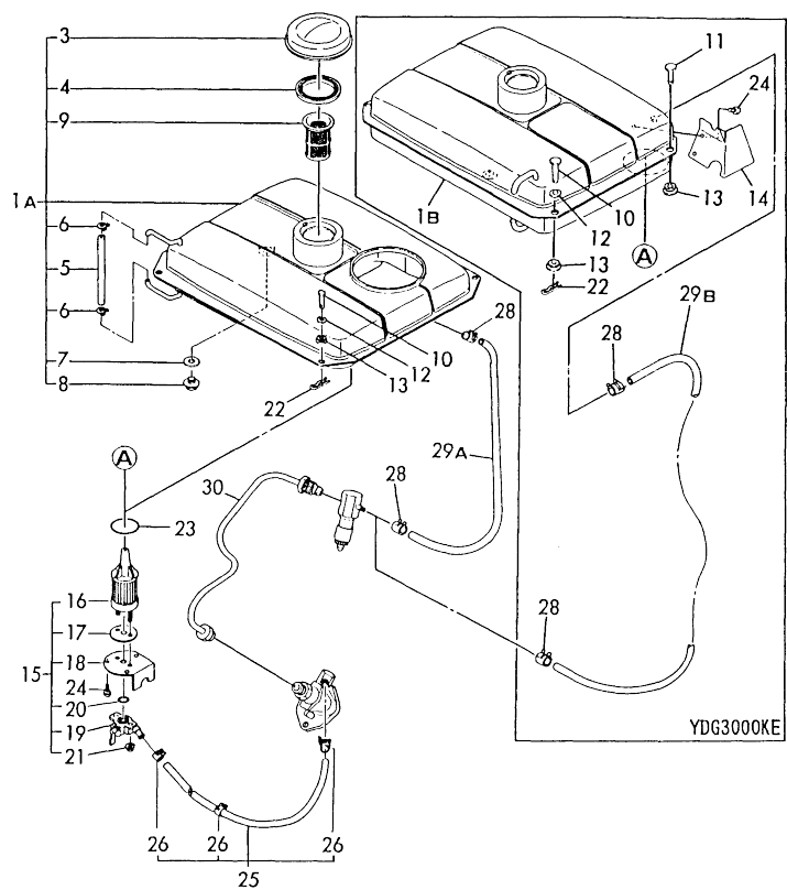
Fig.71 FUEL TANK & FUEL LINE
