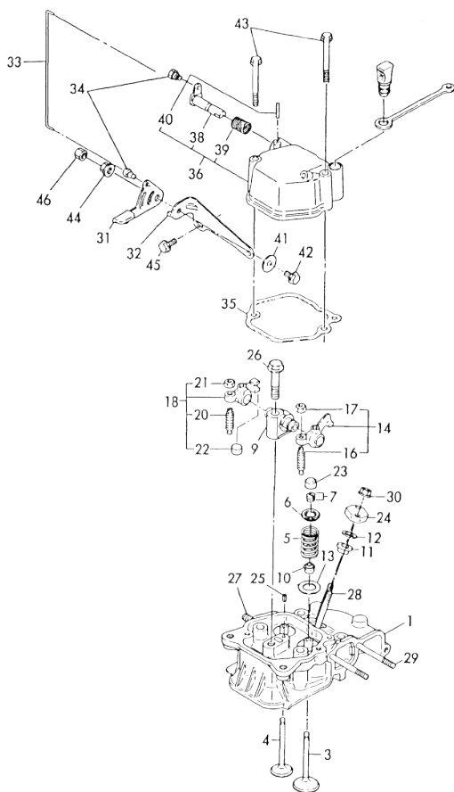
Fig. 64 CYLINDER HEAD
