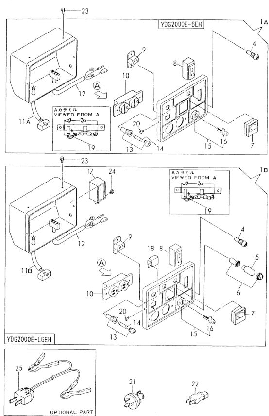
Fig.14 PANEL BOX
