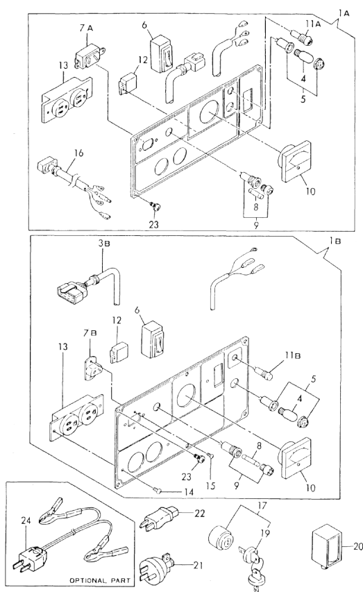
Fig. 90 PANEL
