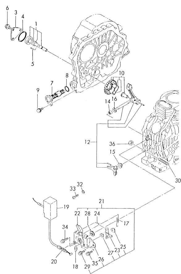
Fig.67 L.O PUMP & ENGINE CONTROL
