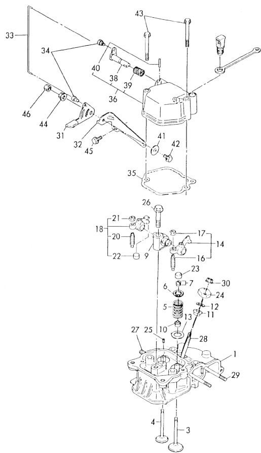
Fig.64 CYLINDER HEAD
