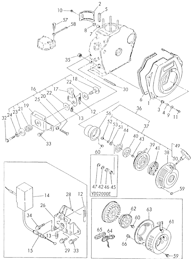
Fig.6 COOLING & STARTING DEVICE
