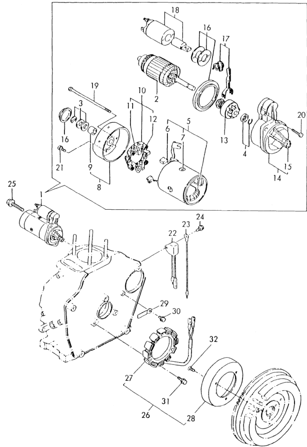
Fig.40 STARTING MOTOR & DYNAMO
