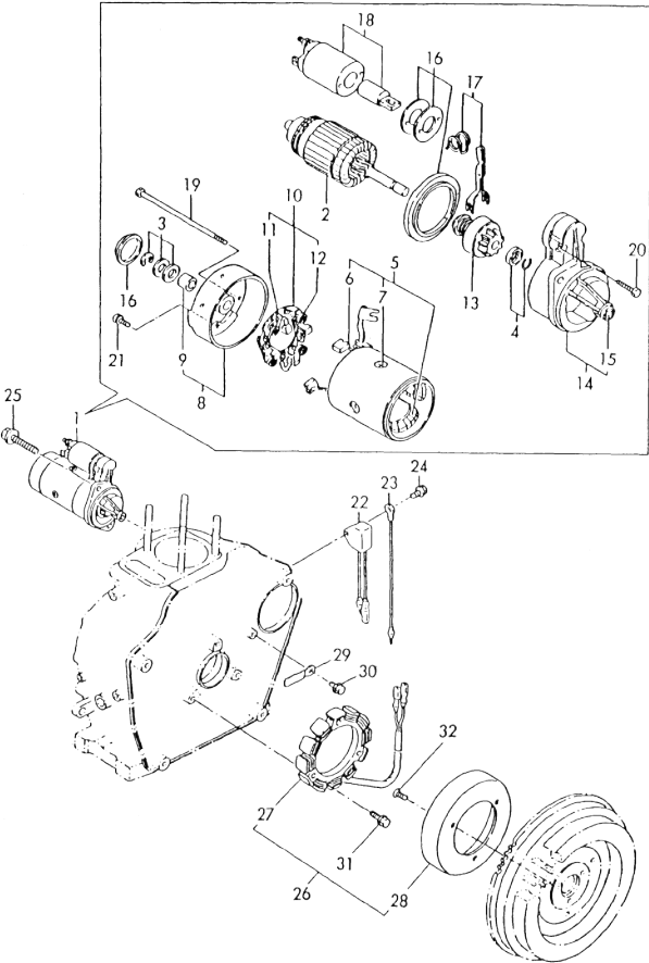
Fig.115 STARTING MOTOR & DYNAMO
