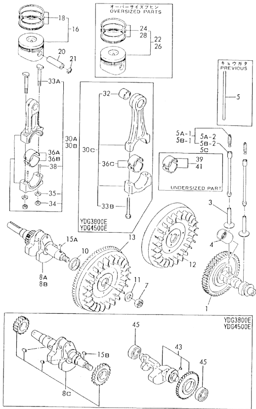
Fig.81 CRANKSHAFT / PISTON/ROD
