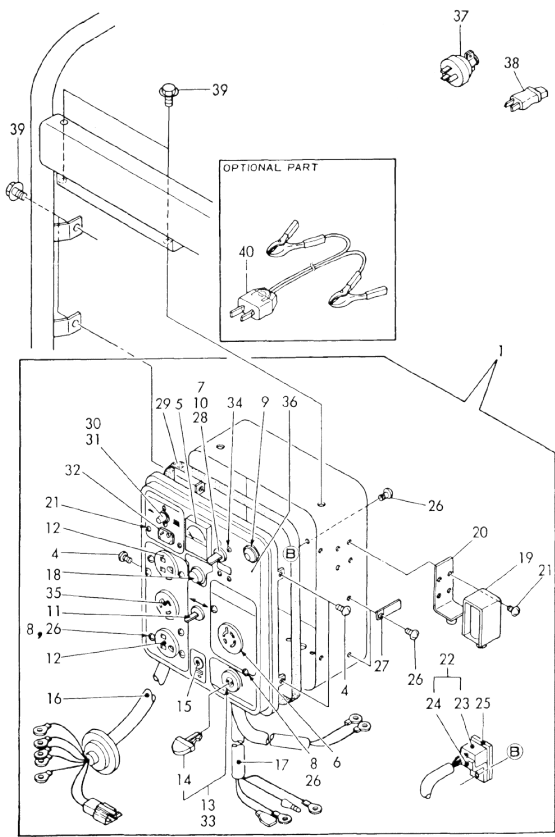
Fig. 31 PANEL BOX
