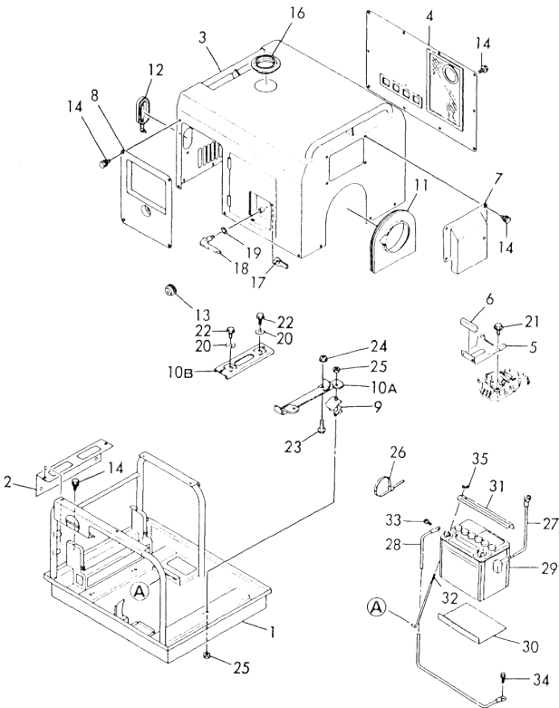
Fig. 75 SOUND-PROOF CASE
