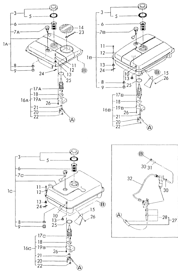
Fig.39 FUEL TANK & FUEL LINE
