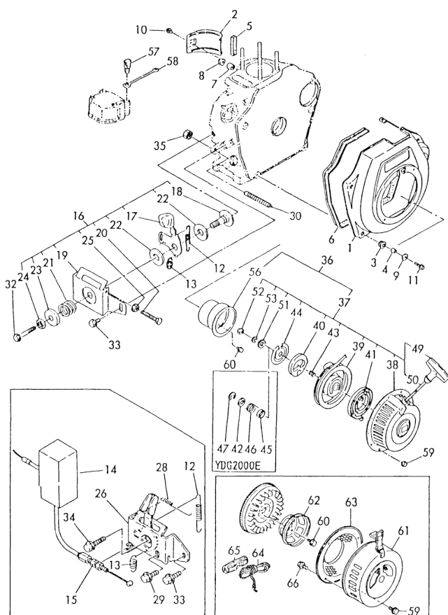
Fig. 37 COOLING & STARTING DEVICE
