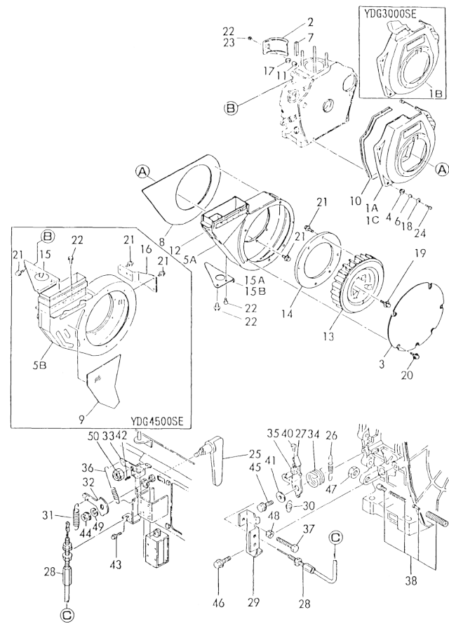
Fig. 96 COOLING & ENGINE CONTROL
