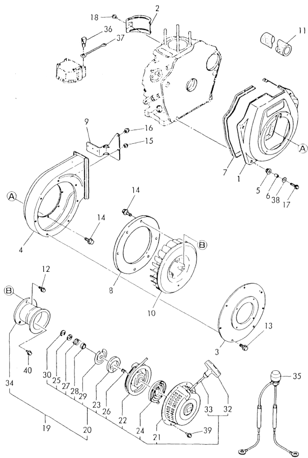
Fig.68 COOLING & STARTING DEVICE
