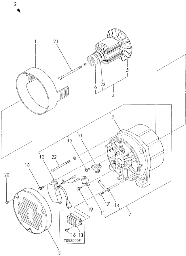
Fig.76 GENERATOR
