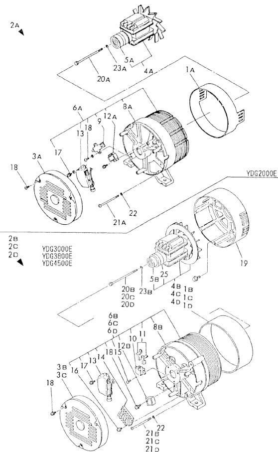
Fig.13 GENERATOR
