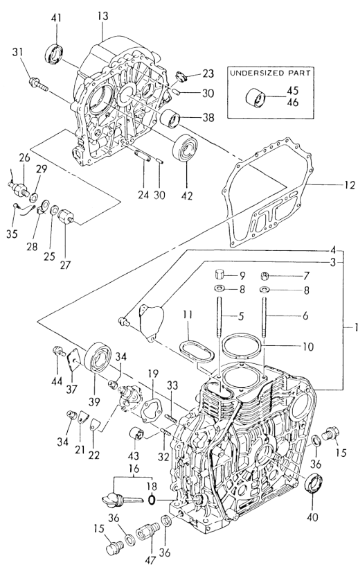
Fig. 63 CYLINDER BLOCK
