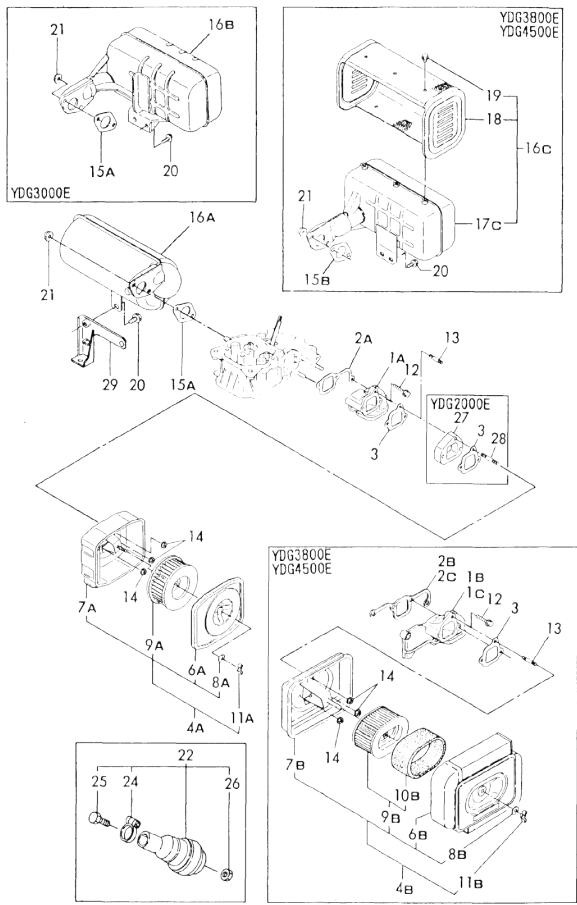
Fig.3 AIR CLEANER & SILENCER
