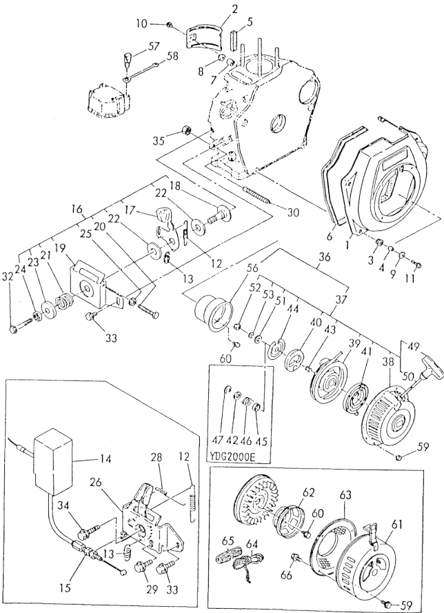
Fig. 21 COOLING & STARTING DEVICE
