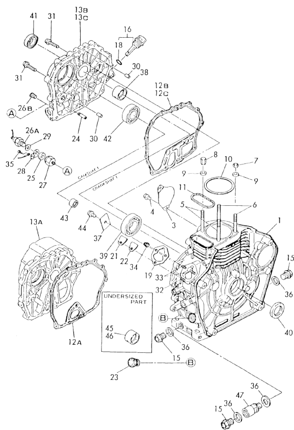
Fig. 107 CYLINDER BLOCK
