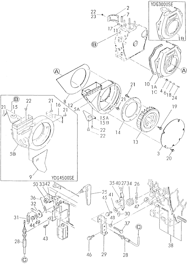
Fig. 112 COOLING & ENGINE CONTROL
