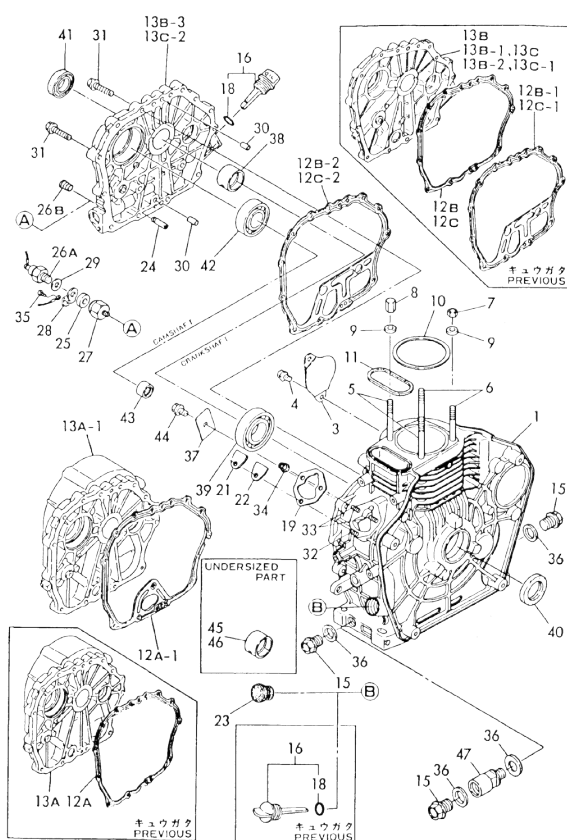
Fig. 78 CYLINDER BLOCK
