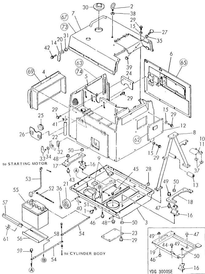
Fig.88 SOUND-PROOF CASE
