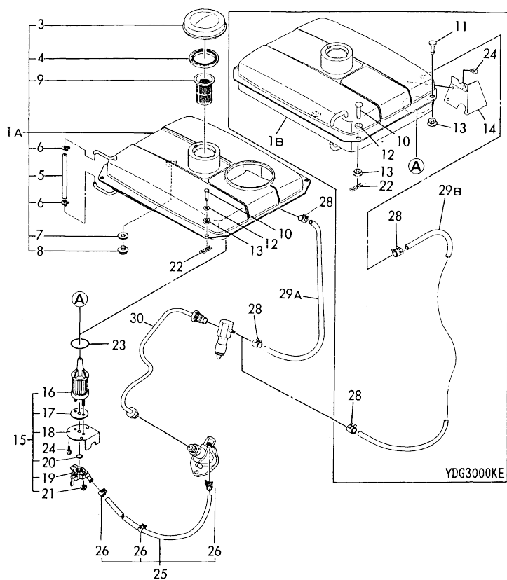
Fig. 56 FUEL TANK & FUEL LINE
