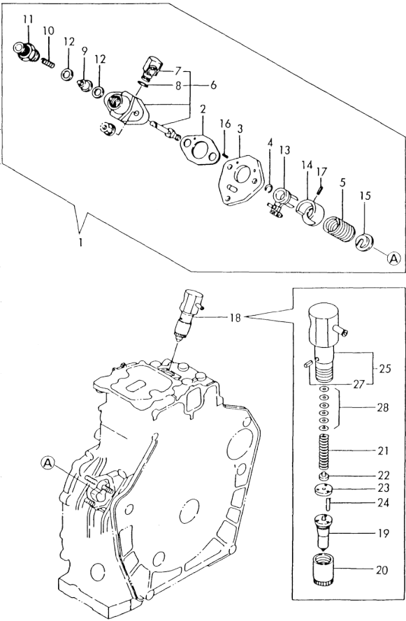
Fig.70 FUEL INJECTION PUMP & VALVE
