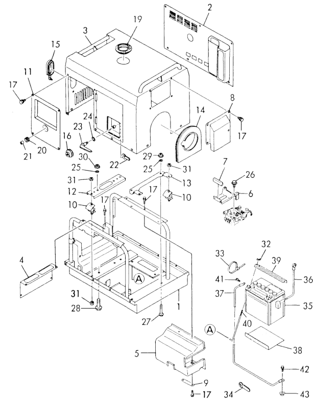
Fig.59 SOUND-PROOF CASE
