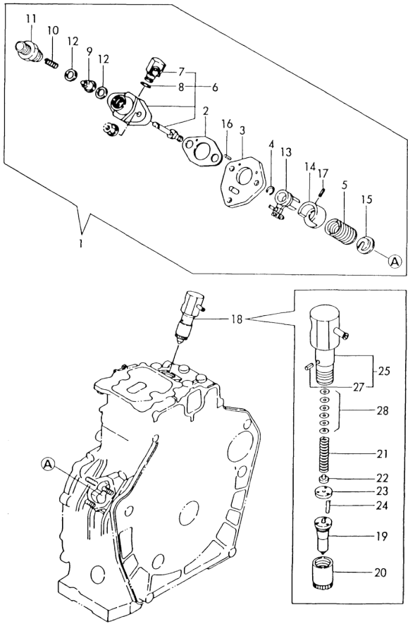
Fig. 55 FUEL INJECTION PUMP & VALVE
