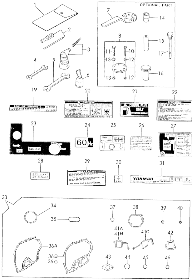
Fig. 100 TOOLS/LABELS & GASKET SET
