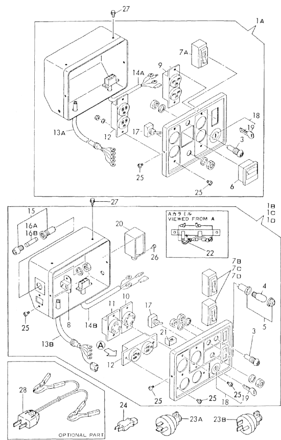
Fig. 15 PANEL BOX
