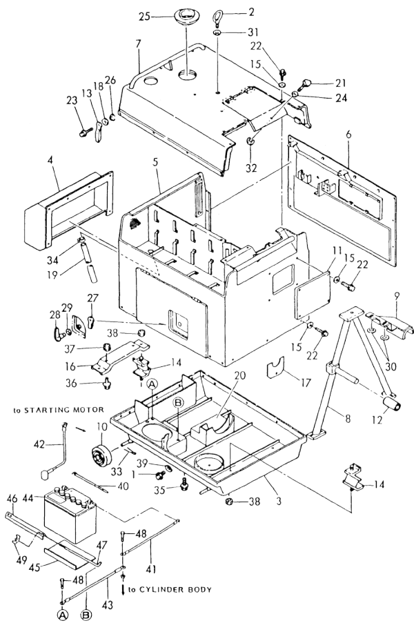
Fig. 118 SOUND-PROOF CASE
