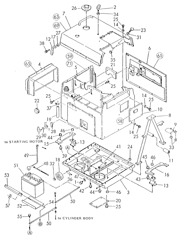
Fig. 117 SOUND-PROOF CASE
