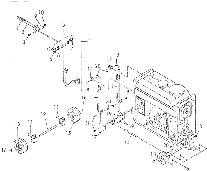
Fig. 27 WHEEL (OPTIONAL PARTS)
