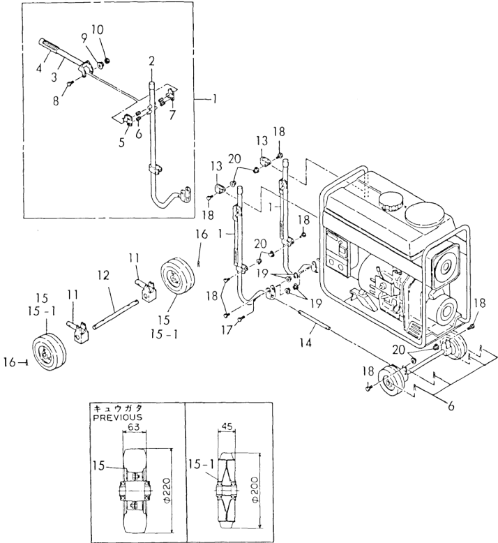
Fig. 12 WHEEL (OPTIONAL PARTS)
