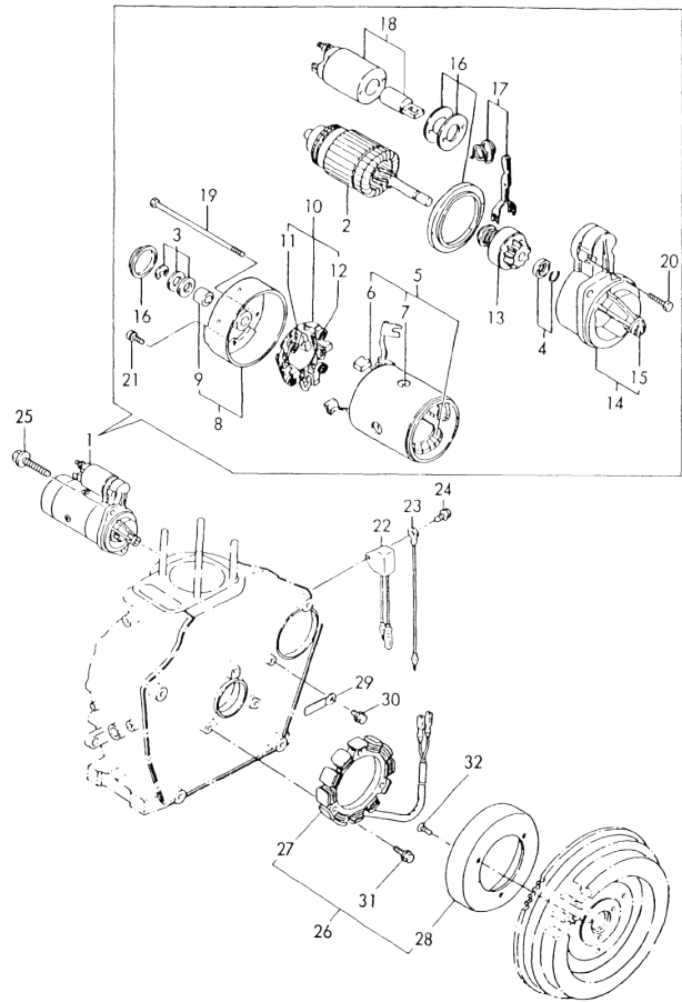
Fig.24 STARTING MOTOR & DYNAMO
