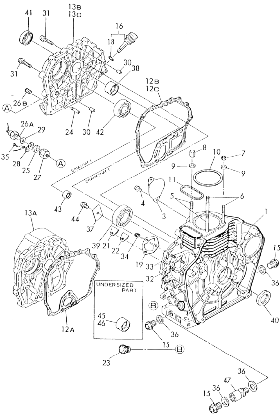
Fig.91 CYLINDER BLOCK
