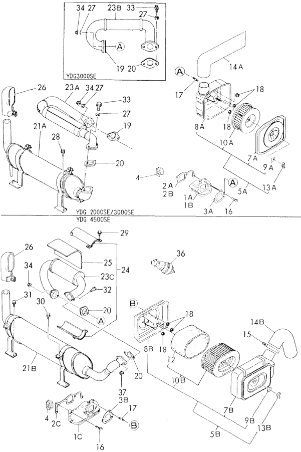
Fig. 80 AIR CLEANER & SILENCER
