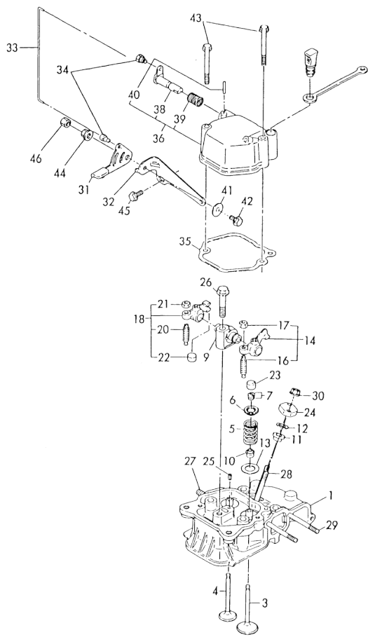
Fig. 33 CYLINDER HEAD
