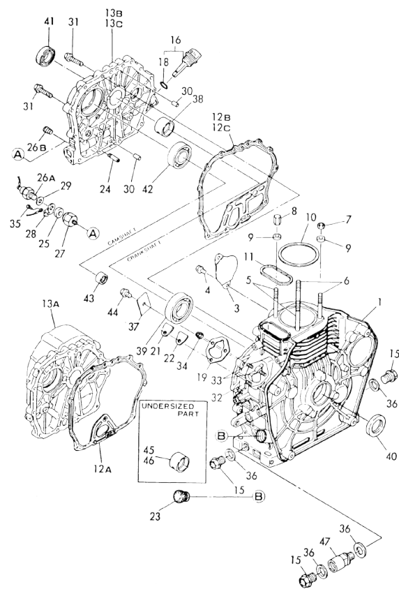
Fig. 16 CYLINDER BLOCK
