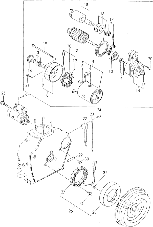
Fig.72 STARTING MOTOR & DYNAMO
