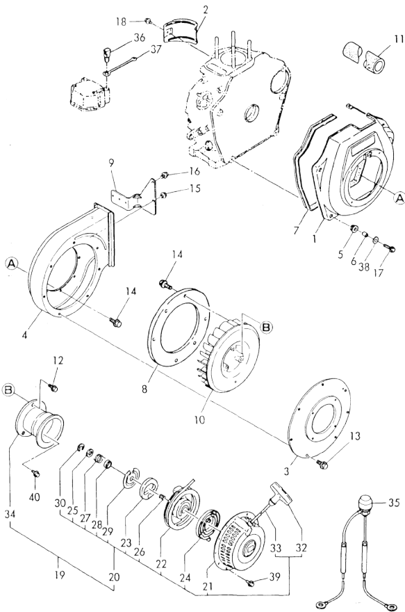
Fig.53 COOLING & STARTING DEVICE
