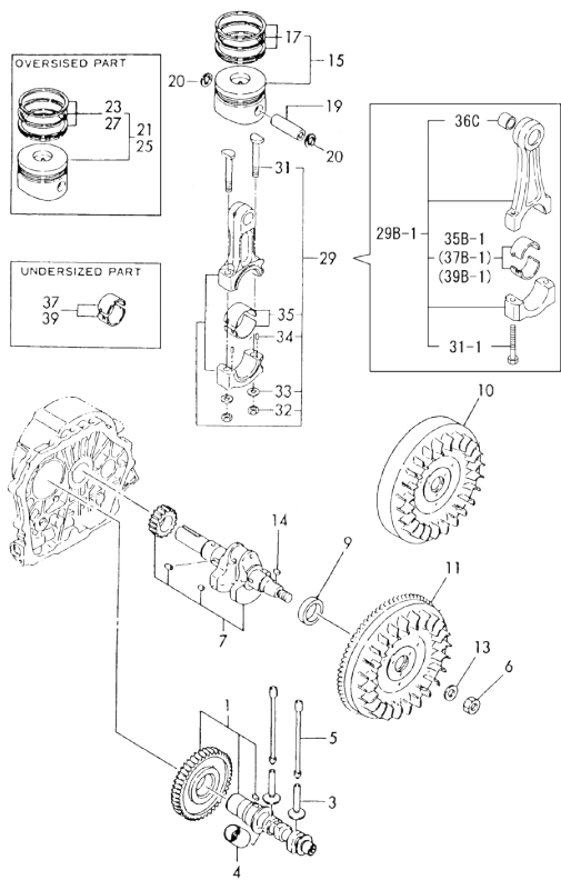
Fig.51 CRANKSHAFT / PISTON / ROD
