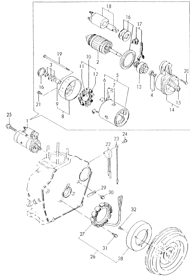
Fig. 9 STARTING MOTOR & DYNAMO
