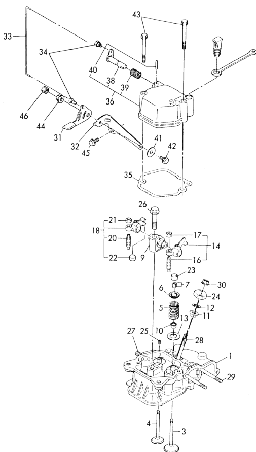
Fig. 49 CYLINDER HEAD
