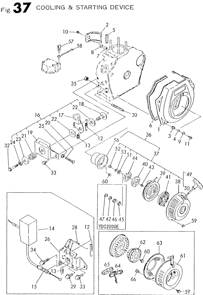
Fig.37. COOLING & STARTING DEVICE
