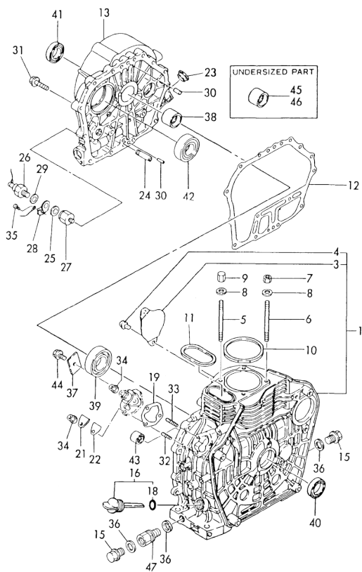
Fig.48 CYLINDER BLOCK
