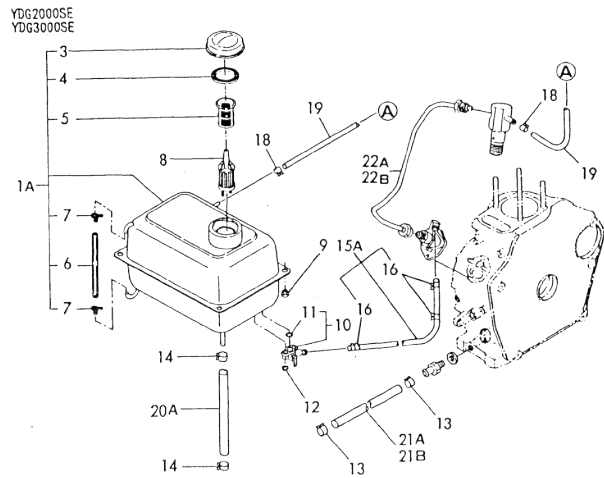
Fig. 114 FUEL TANK & FUEL LINE
