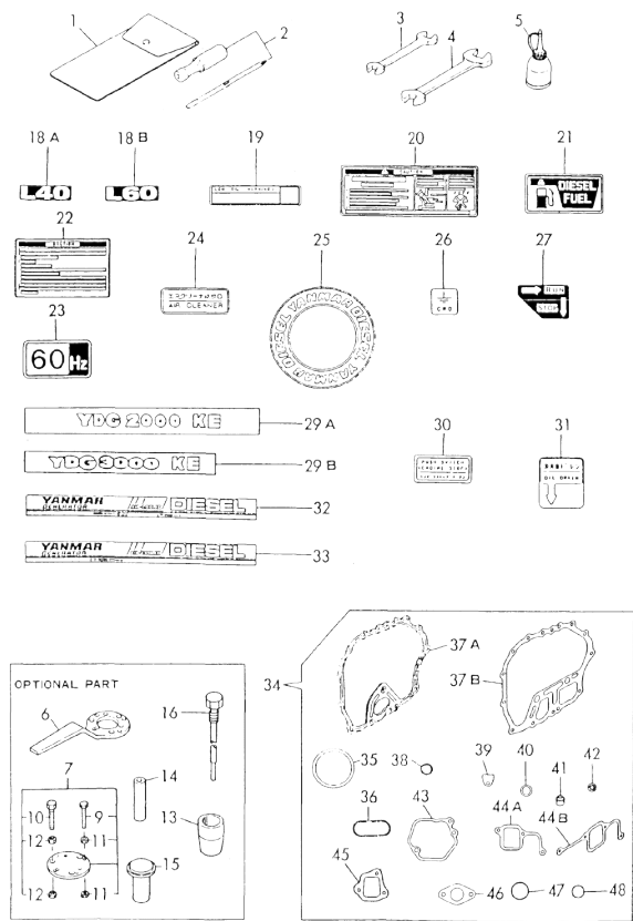
Fig.58 TOOLS/LABELS & GASKET SET
