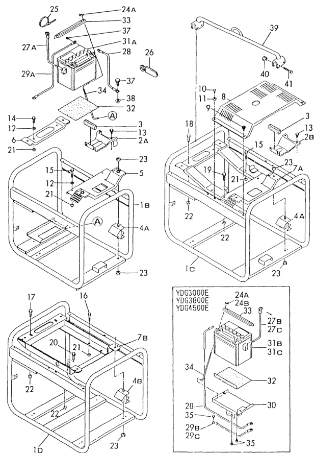
Fig.42 FRAME & BATTERY
