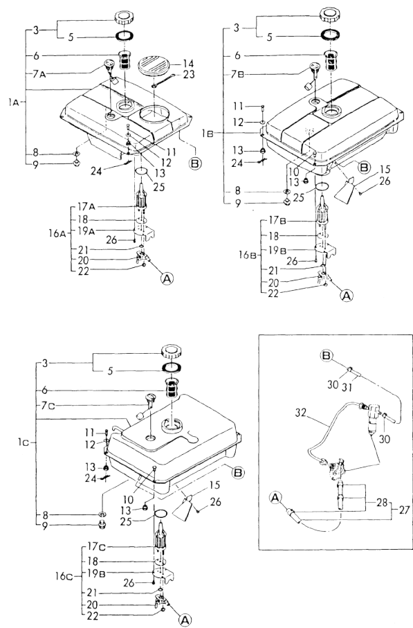
Fig.23 FUEL TANK & FUEL LINE
