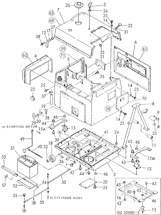
Fig.101 SOUND-PROOF CASE
